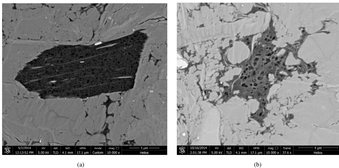
Fig. 8. Shale microscopic imaging in Longmaxi formation in Chongqing.
