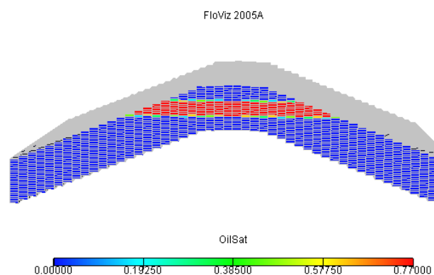
Fig. 1. Anticlinal oil rim reservoir.
