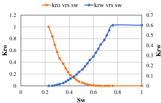
Fig. 2. Oil-Water relative permeability curve.
