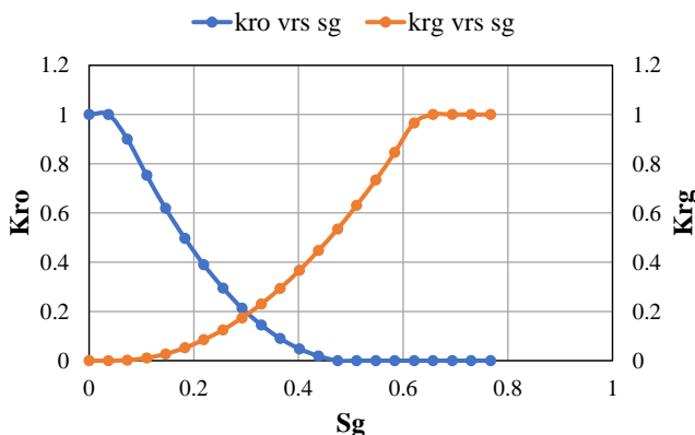
Fig. 3. Gas-Oil relative permeability curve.
