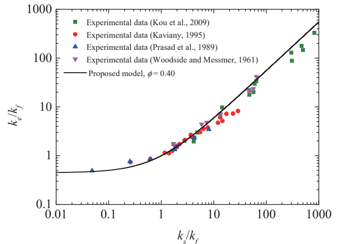
Fig. 3. The comparison between proposed model prediction and experimental data for saturated porous media when the porosity equals to 0.40, where \alpha = 0.01 , \beta = 0.01 , 2(h_{\max})_{\lambda_{\min}}/\lambda_{\min} = 0.1 and \varphi = 0.2 .
